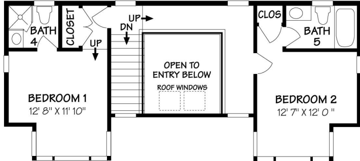
UPPER FLOOR
